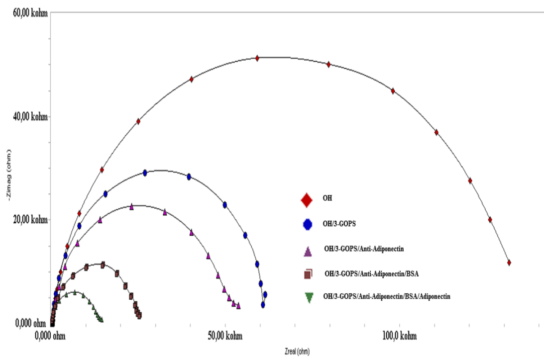
Figure 2. Nyquist plots for immobilization steps
