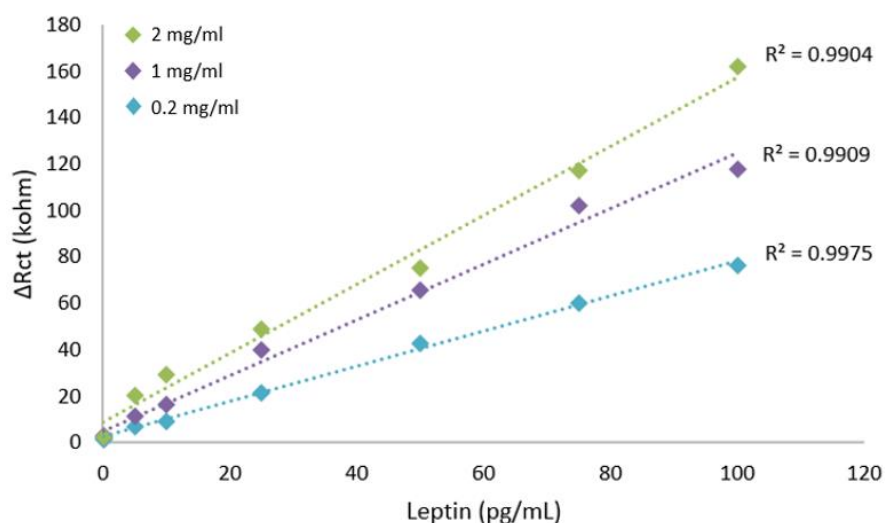
Figure 3. Standard curves for Leptin obtained by different CNBr concentrations
