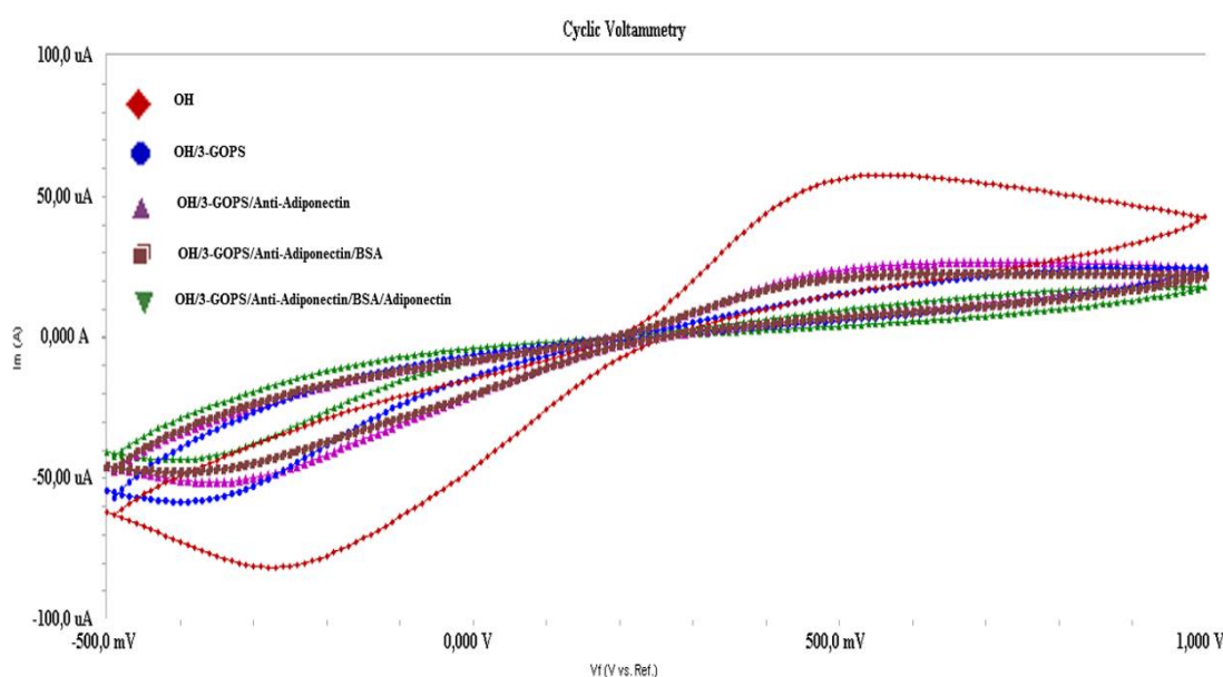
Figure 3. Cyclic voltammograms for immobilization steps of Anti-Adiponectin
