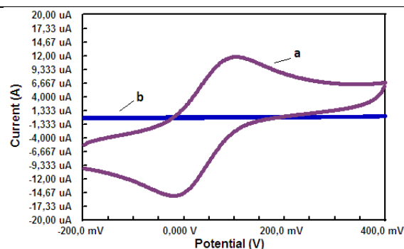
Fig. 2. The comparison of cyclic voltammograms of 1.0 mM of Fe(CN) 6 3- in BR buffer (pH=2.0) of (a) bare GC and (b) BODIPY-I/GC electrodes..
