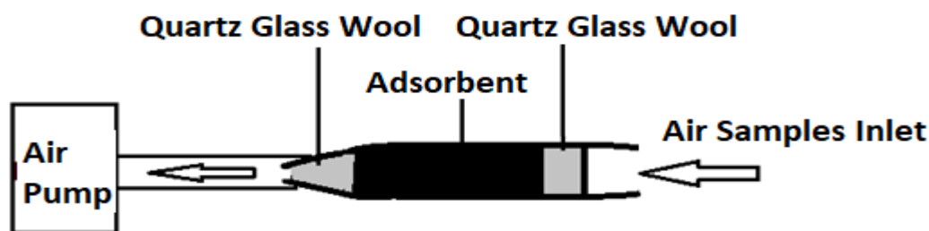
Figure 1. Air sampling of targeted VOCs
