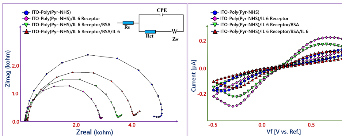
Figure 1. EIS and CV responses obtained during immobilization steps.
